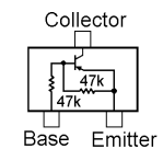
RT1P441U (P3) (Q1013, 1020, 1059)
