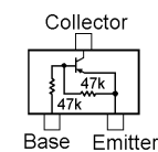
RT1P441U (P3) (Q1013, 1020, 1059)
