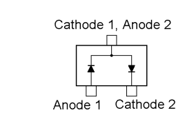
MC2850 (A7) (D1030)
