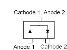
MC2850 (A7) (D1030)
