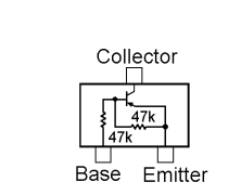
RT1P441U (P3) (Q1013, 1020, 1059)
