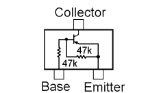
RT1P441U (P3) (Q1013, 1020, 1059)
