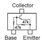
RT1N441U (N3) (Q1034, 1045, 1063)
