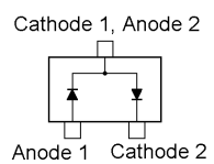
MC2850 (A7) (D1015, 1031, 1032, 1034)
