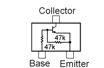
RT1P441U (P3) (Q1013, 1020, 1059)
