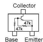
RT1N441U (N3) (Q1034, 1045, 1063)
