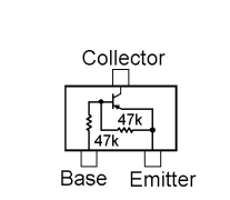
RT1P441U (P3) (Q1013, 1020, 1059)
